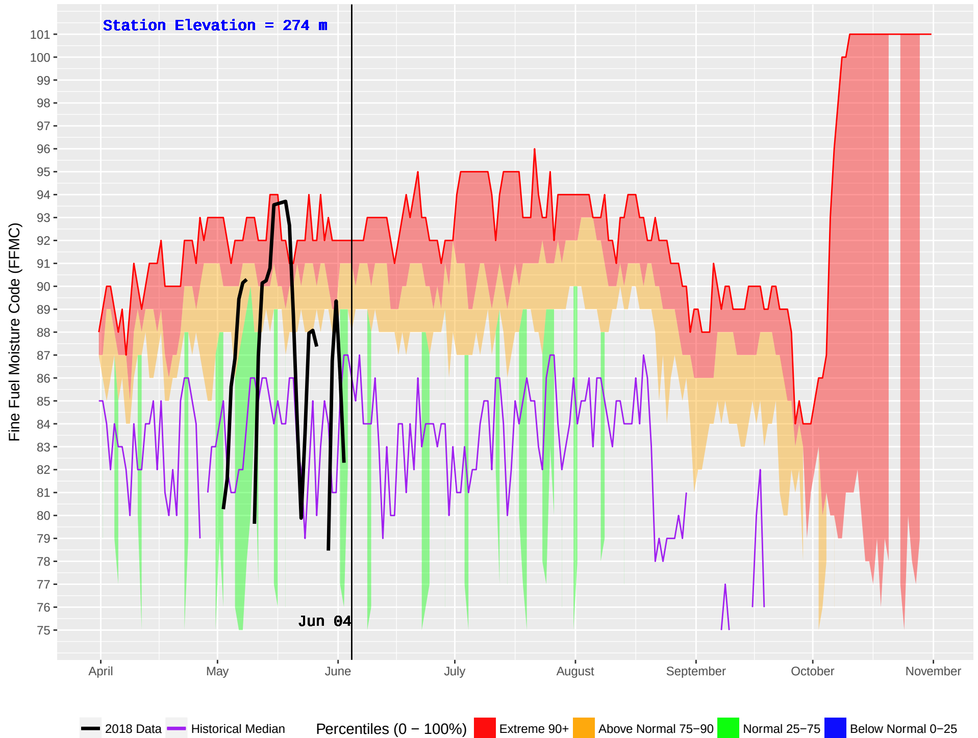
CEDARVALE (429) : Historical (1982–2016) and Current (2018) Noon Fine Fuel Moisture Code (FFMC)
