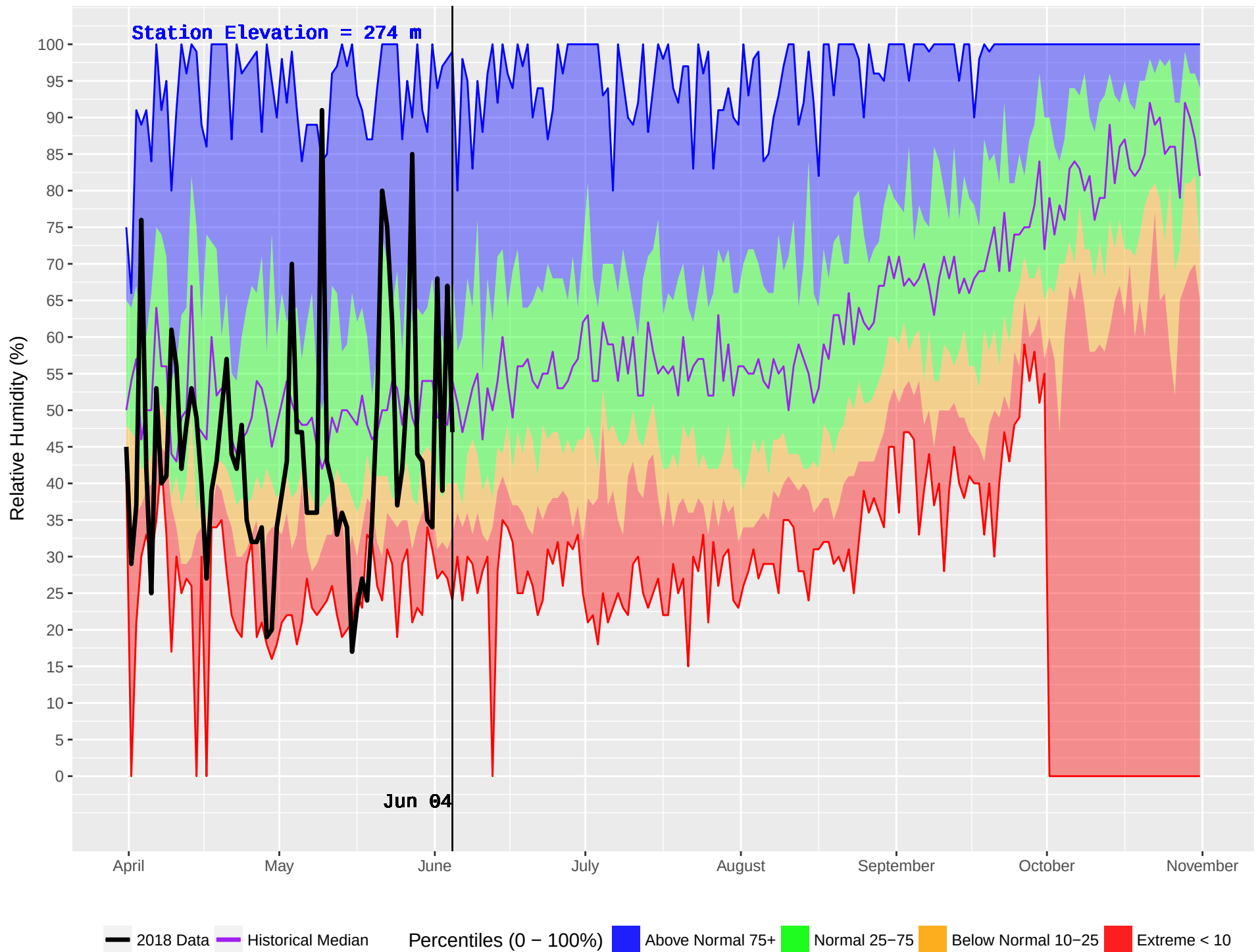
CEDARVALE (429) : Historical (1982–2016) and Current (2018) Noon Relative Humidity
